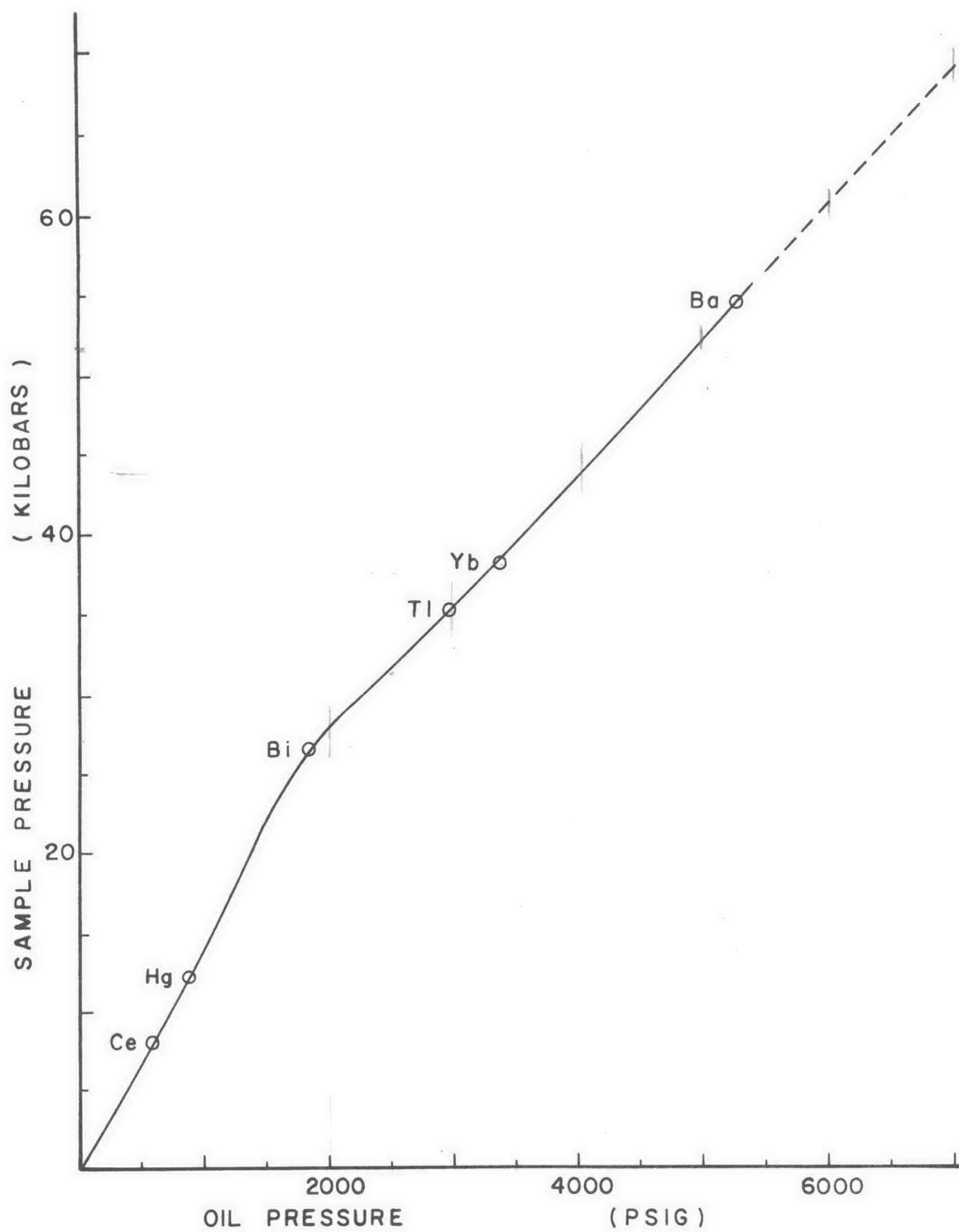
Fig. 24.--Pressure Calibration
